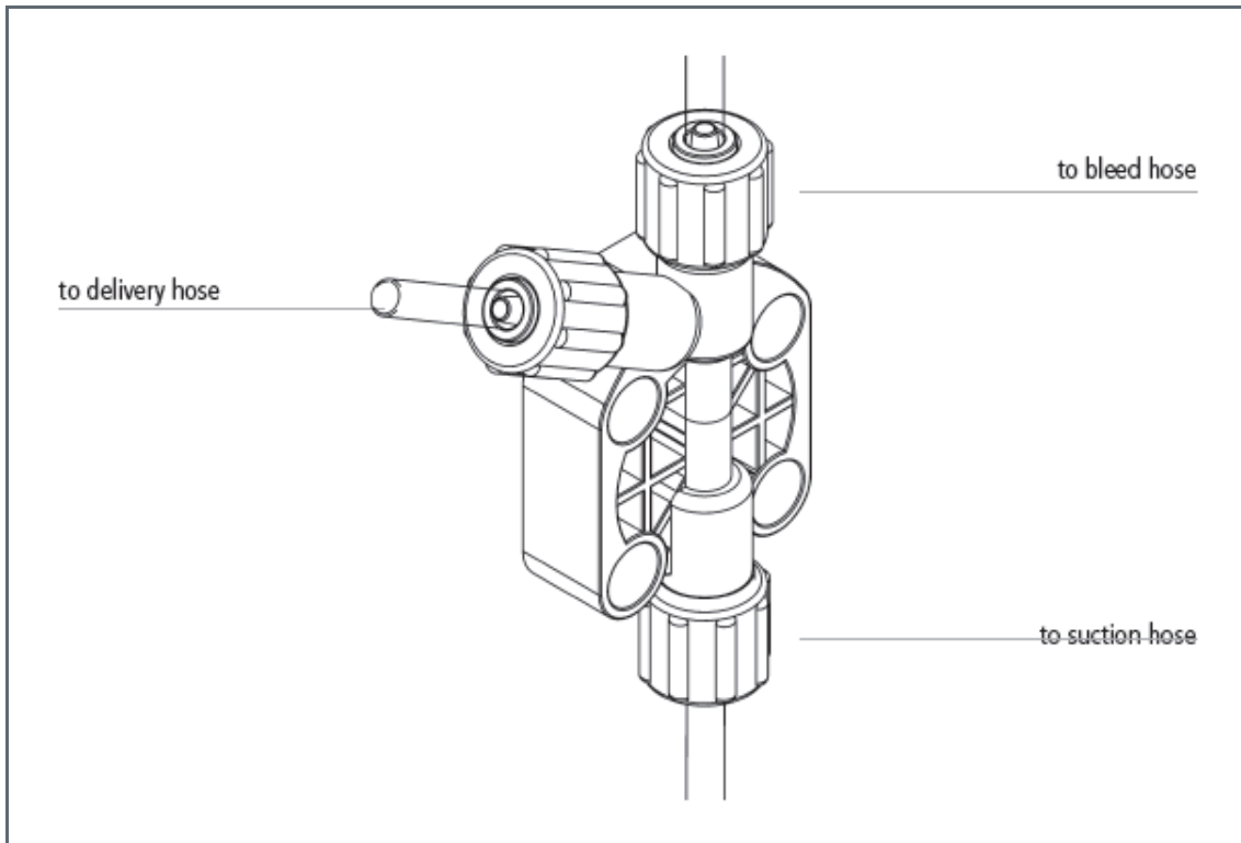
Figure 8 Self-venting models pump head
