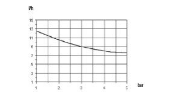
057.5: I/h 7.5 bar 5 Pump head mod. KA
