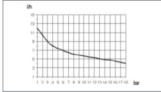
1804: l/h 4 bar 18 Pump head mod. K
