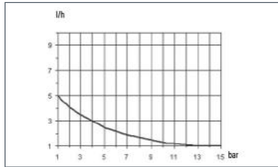
1501: I/h 1 bar 15 Pump head mod. KA
