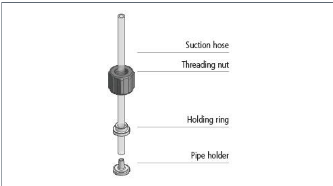
Figure 5 Suction hose assembling
