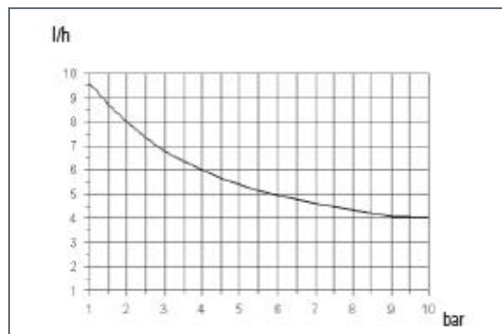
1004: l/h 4 bar 10 Pump head mod. K
