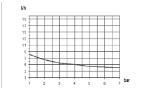
0704: I/h 4 bar 7 Pump head mod. KA
