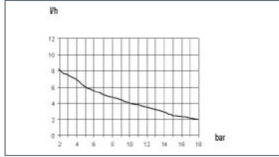
1802: I/h 2 bar 18 Pump head mod. KA
