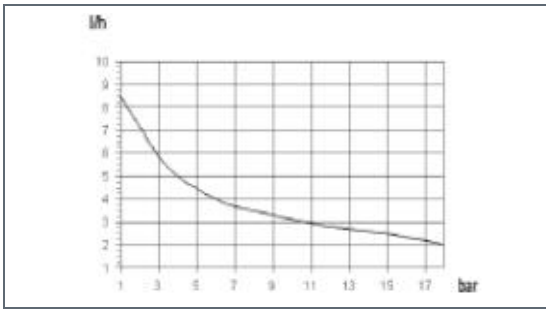
1802: l/h 2 bar 18 Pump head mod. K
