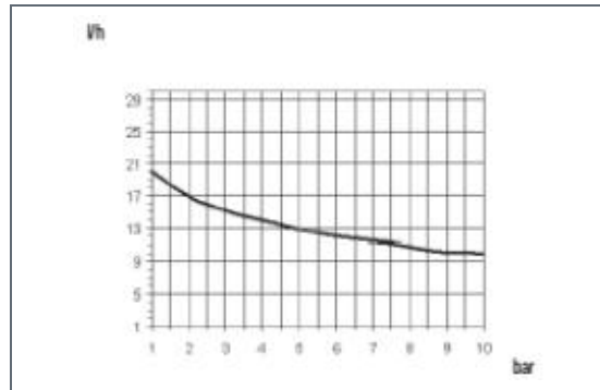
1010: l/h 10 bar 10 Pump head mod. K
