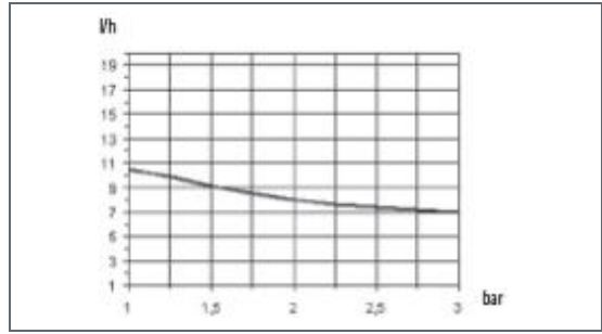
0307: l/h 7 bar 3 Pump head mod. KA
