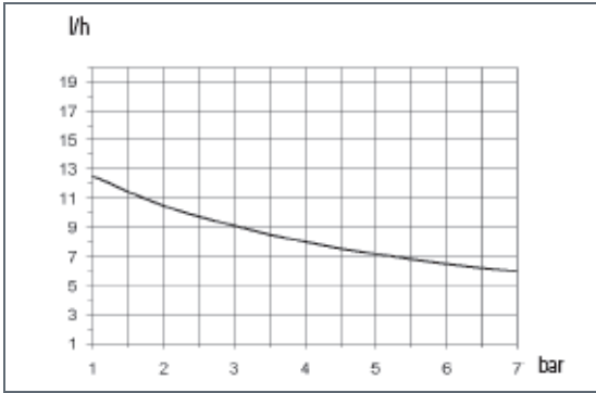
0706: l/h 6 bar 7 Pump head mod. K
