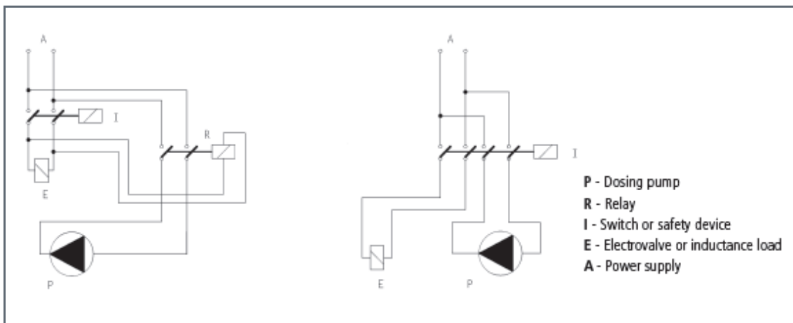
Figure 9 Electrical installation.
