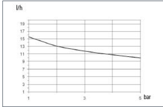
0510: l/h 5 bar 10 Pump head mod. K
