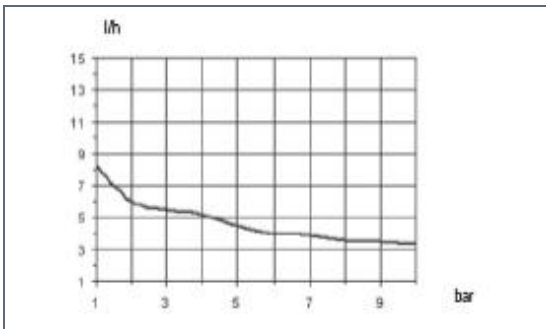
103.4: I/h 3.4 bar 10 Pump head mod. KA
