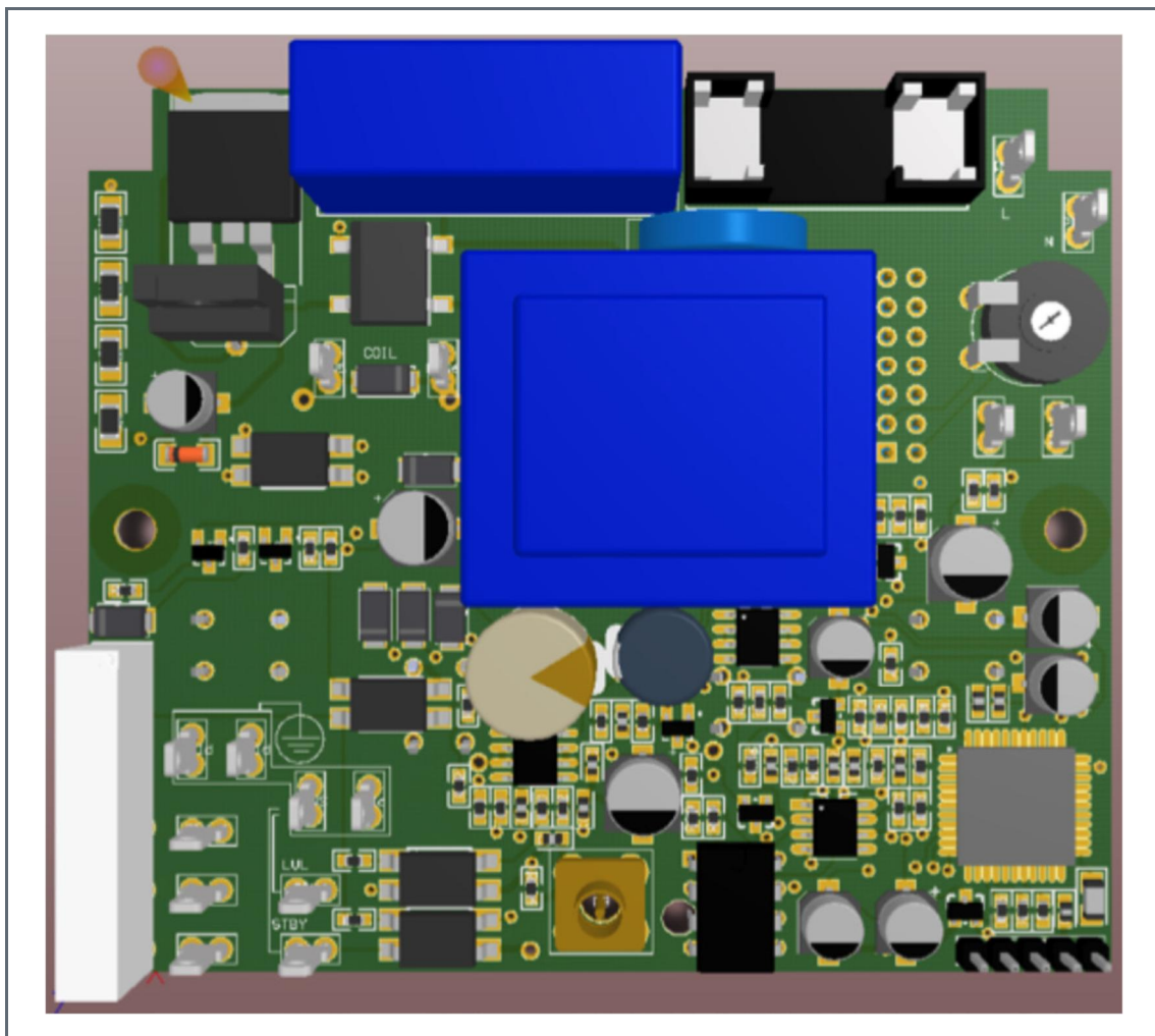
Figure 11 Main board scheme
