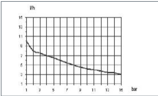
1503: I/h 3 bar 15 Pump head mod. KA
