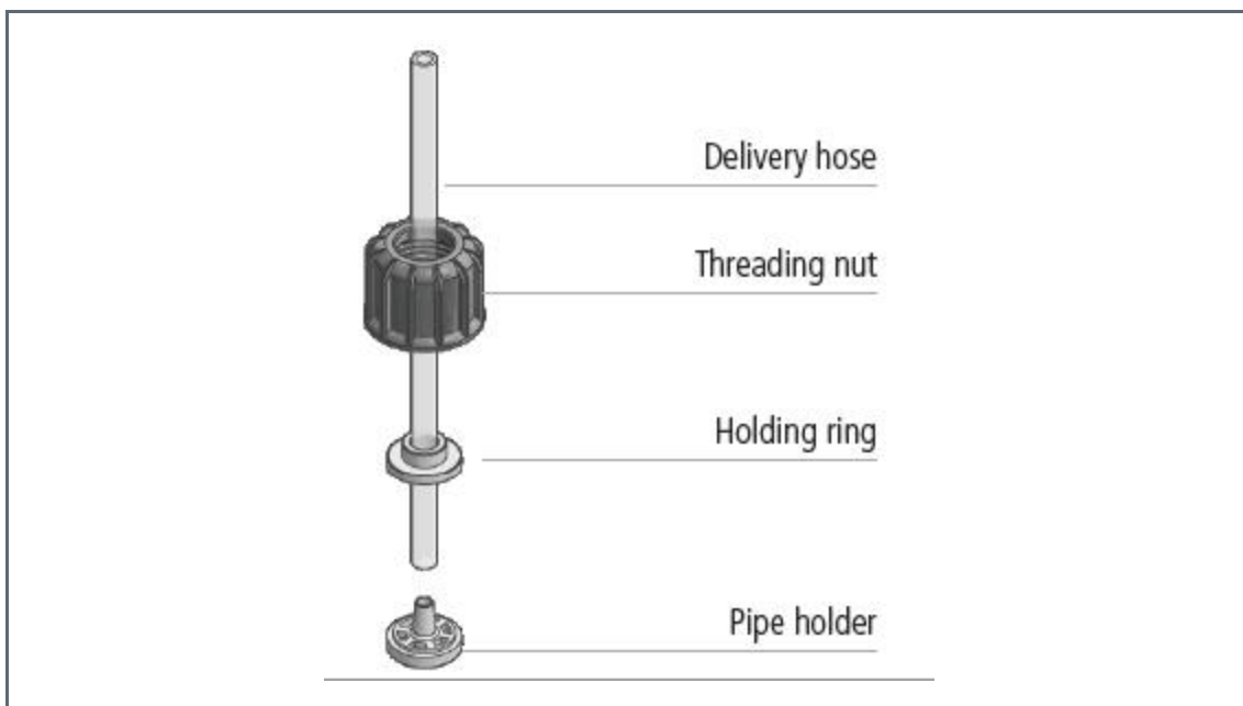
Figure 6 Delivery hose / pump head assembling
