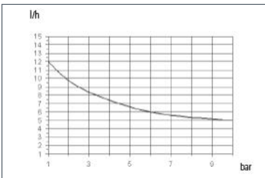
1005: l/h 5 bar 10 Pump head mod. K
