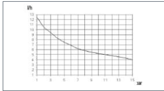
1504: l/h 4 bar 15 Pump head mod. K
