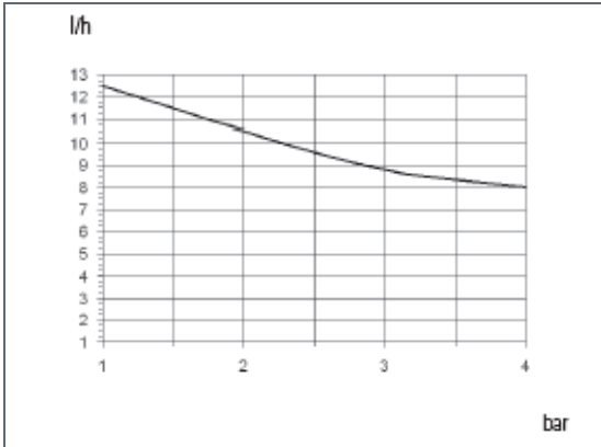
0408: l/h 8 bar 4 Pump head mod. K
