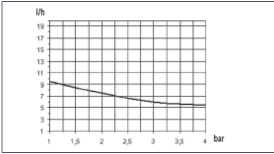
045.5: l/h 5.5 bar 4 Pump head mod. KA
