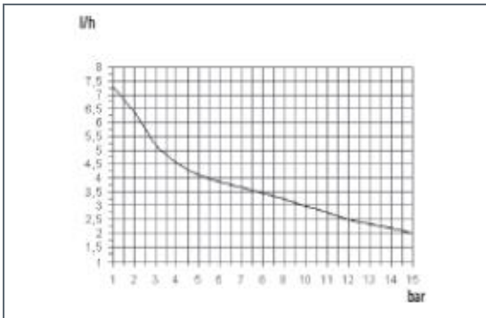
1502: l/h 2 bar 15 Pump head mod. K
