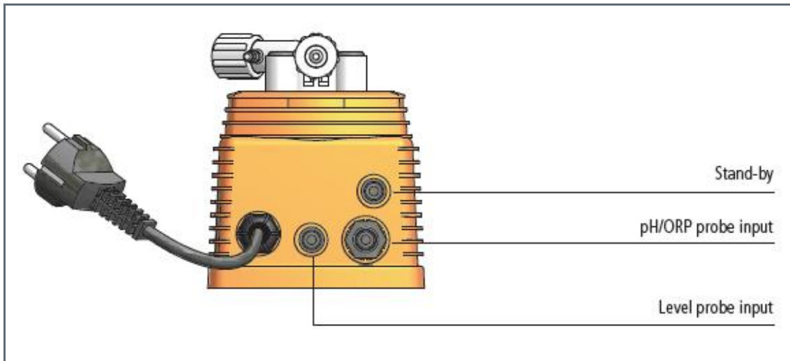
Figure 10 Wirings
