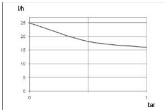
0116: l/h 16 bar 1 Pump head mod. K
