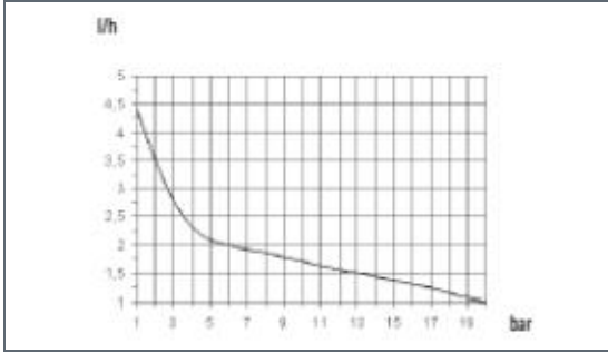
2001: l/h 1 bar 20 Pump head mod. J
