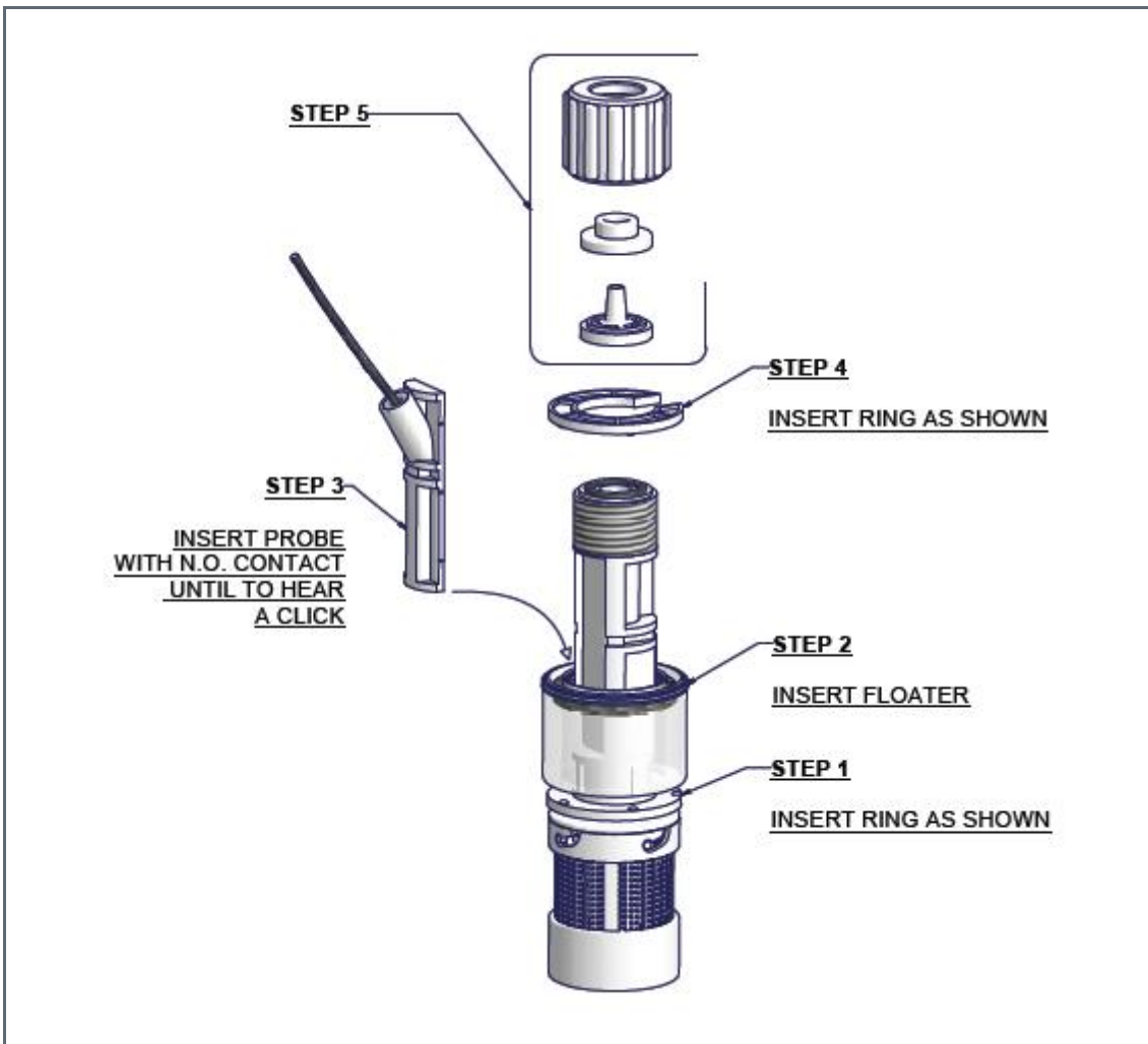
Figure 4 Level probe assembling diagram.
